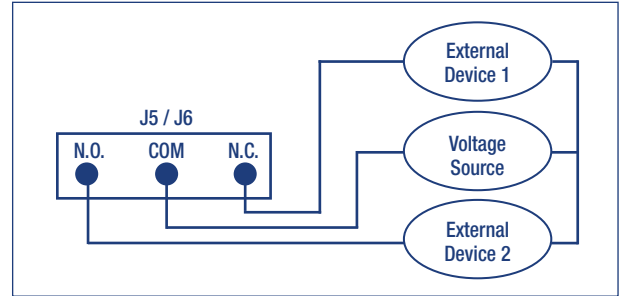
Figure 6 Wiring Diagram for External Power Relays
